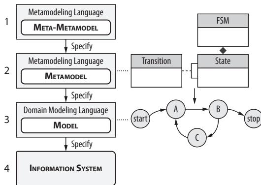
Figure 1: Four-layer metamodeling
